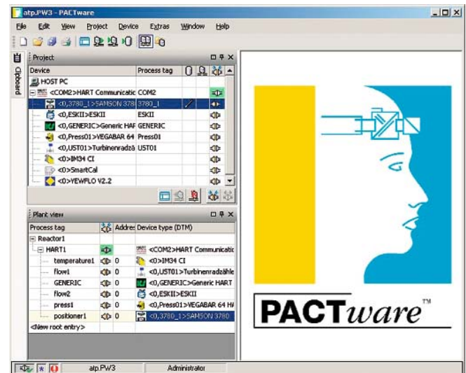
Network and plant view of a project
